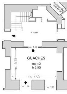
Piano Terra / Ground Floor
